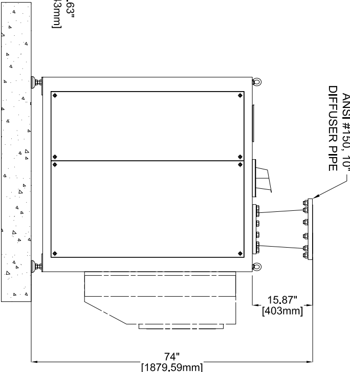
VIEW "D" (RIGHT SIDE)
