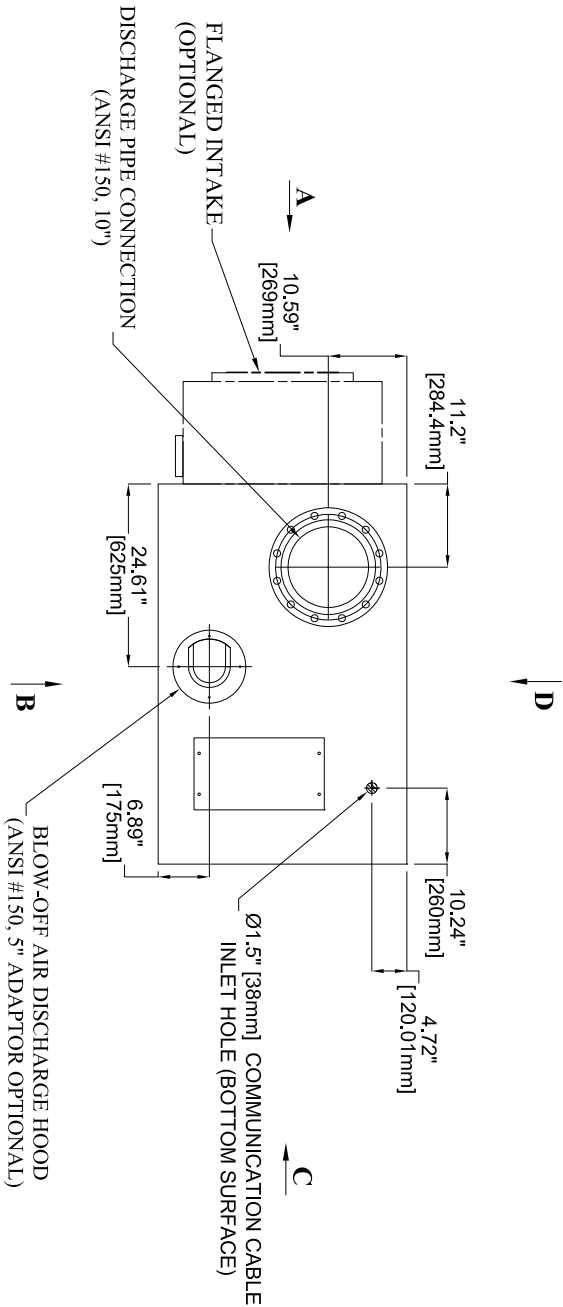
VIEW "E-E" (LOOKING DOWNWARD)
